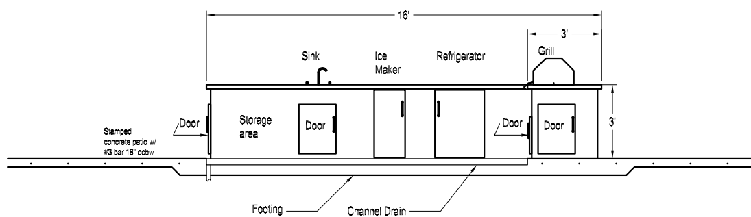
3 Outdoor Kitchen Detail, side view Scale: 1/2" = 1'-0"
